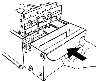
Slide note tray into dispenser mechanism.
